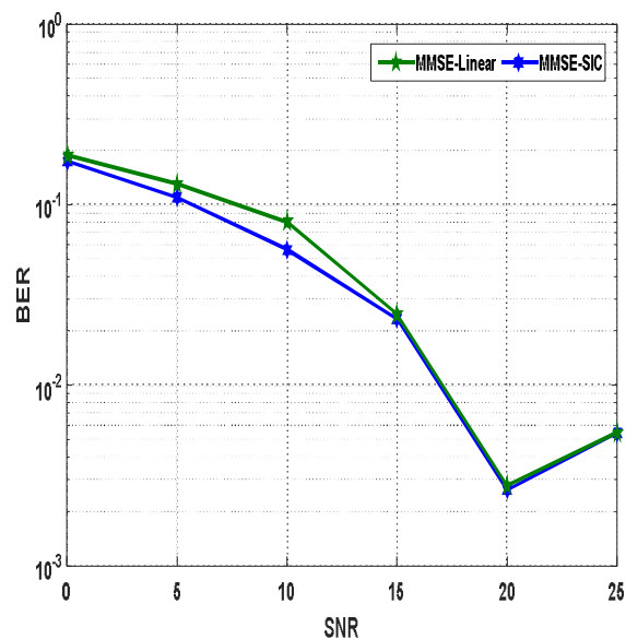
Figure 6 BER against SNR for M = 8, K = N = 2
