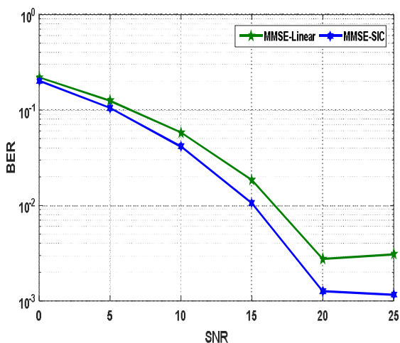
Figure. 8: BER against SNR for M = 8, K = N = 8
