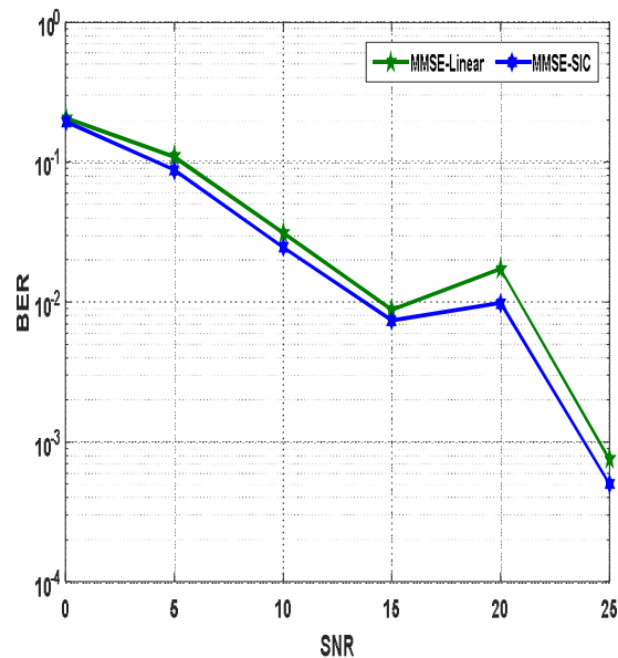
Figure 5: BER against SNR M = 4, K = N = 4
