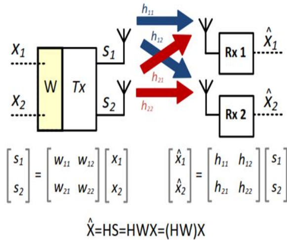
Figure 2: Architecture and channel matrix of MU-MIMO [8] During the channel coherence time, computing W requires that a number of uplink pilots are simultaneously transmitted by all the UEs. The transmitted uplink pilots are received by all BS antennas and then perform pre-weighting matrix computation. Data streams are precoded using measured magnitude and phase on account of the distance from each UE to each of the antenna array. The measured magnitude and phase are also used for distribution of data streams to each antenna port. Thus, the multiuser spatial layer separation does not need to be carried out by the receiver and each UE receives the data separately from the other UEs with better signal to interference-plus-noise ratio (SINR) [8]
