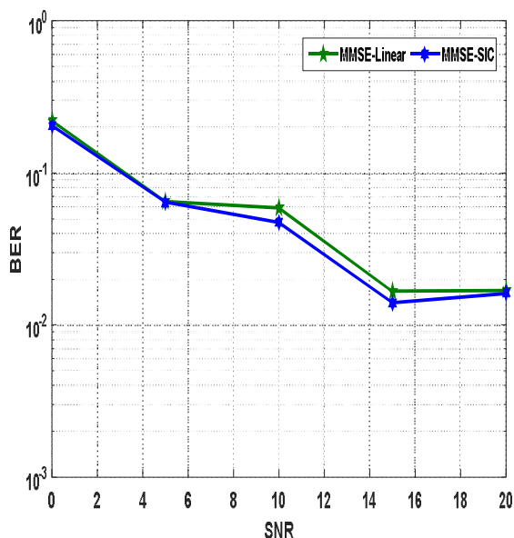
Figure 4: BER against SNR for M = 4, K = N = 2
