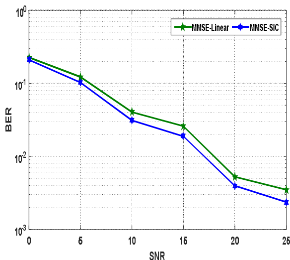
Figure. 7: BER against SNR for M = 8, K = N = 4
