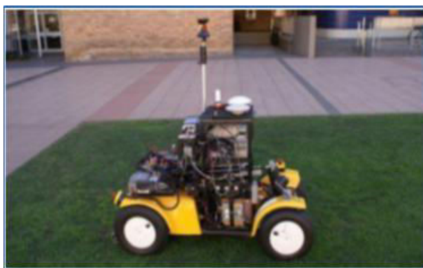
Figure 3: Integrated GPS+INS+Locata test car on UNSW campus.
