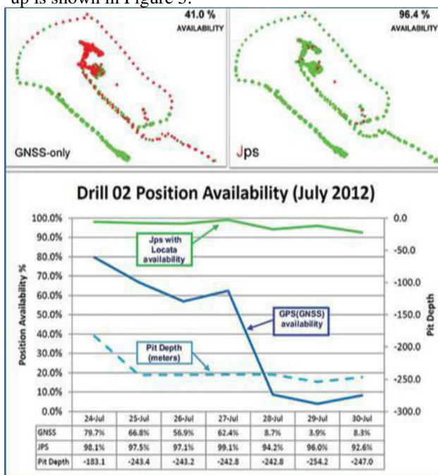
Figure 4: Typical example of position availability for a drill rig operating in a pit at Newmont Boddington Gold mine over a 1-week period in July 2012. Locata-enabled positioning is compared directly against high-accuracy GPS-only availability.
