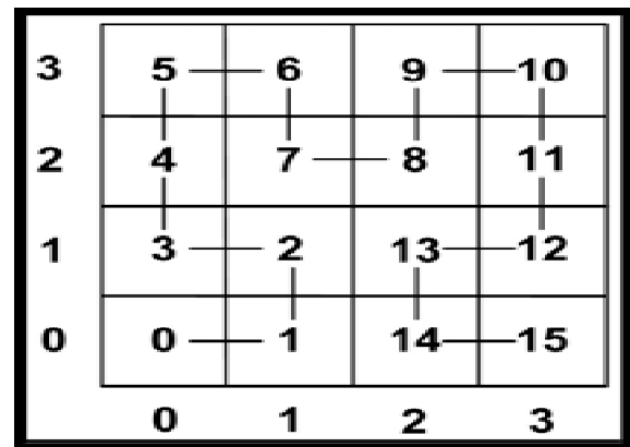
Fig. 1. The Hilbert-curve-based index structure. The numbers represent index values.
