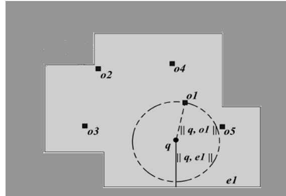
Fig. 3. Because e_1 has the shortest distance to q and \|q, o_1\| \leq \|q, e_1\| , POI o_1 is verified as a valid NN of MH q .
