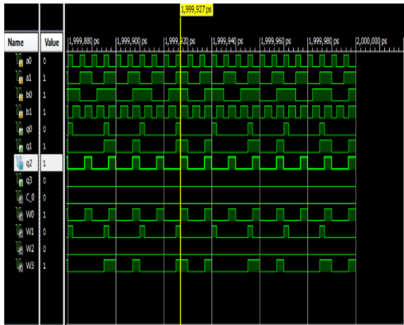
Fig.10: Simulation results for reversible 2*2 Vedic multiplier.
