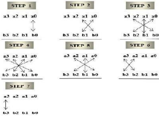
fig.4: multiplication of two 4 bit numbers using urdhvatiryakbhyam.
