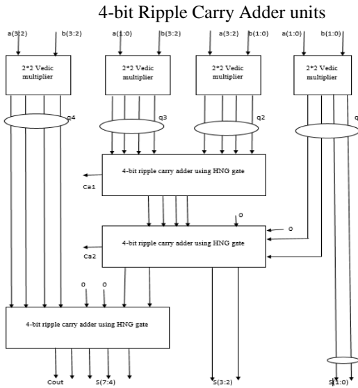
Fig.9: Block diagram of Reversible 4*4 Vedic multiplier.
