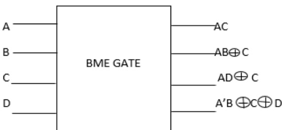
Fig.3: BME gate.
